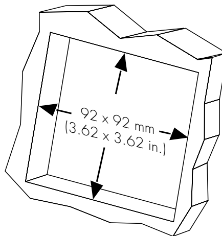
Panel cutout
