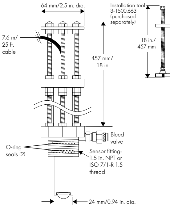
2540/2517 Hot-Tap for 1.5 to 36 in. pipes
